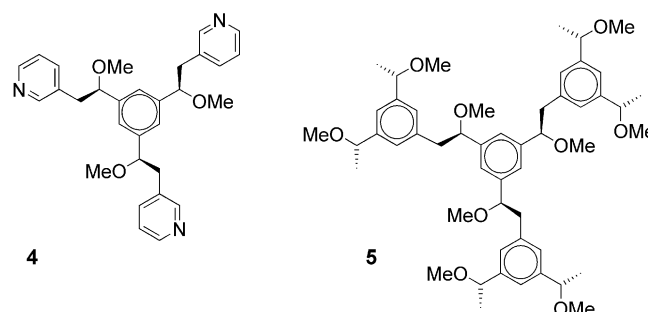
Figure 1. Examples of molecules made using chiral base chemistry.
