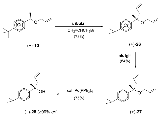
Scheme 7. Synthesis of an enantiopure tertiary alcohol.
