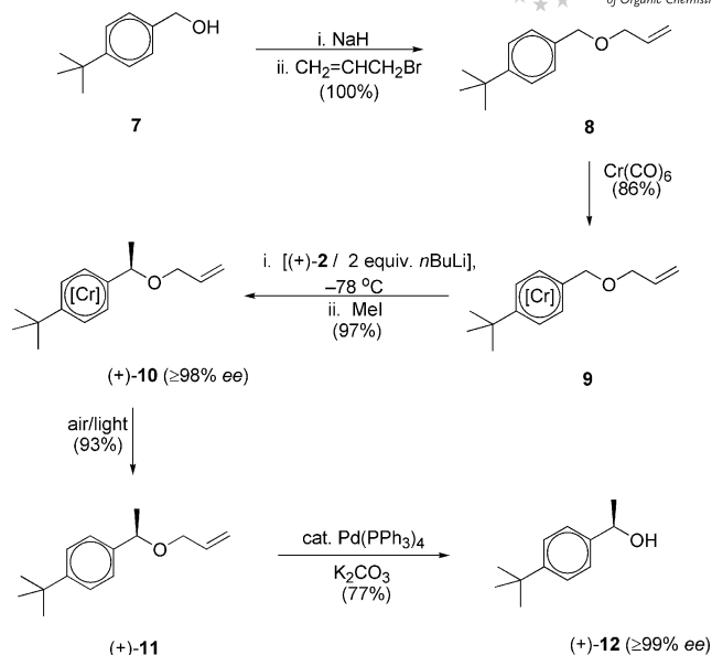
Scheme 3. Use of an allyl ether leads to high selectivities for methylation and the protecting group is readily removed without loss of enantioselectivity [(+)-series depicted here].
