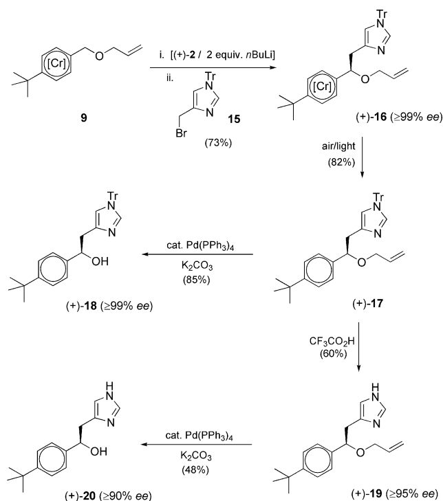
Scheme 5. Synthesis of two imidazole alcohols.
