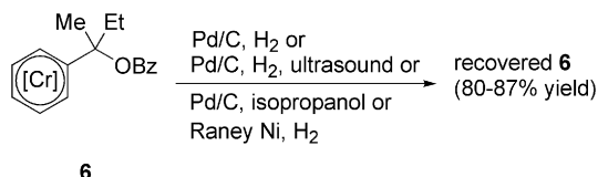
Scheme 2. An early attempt to convert a benzyl ether to its alcohol.
