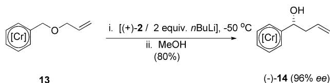
Scheme 4. Deprotection at a higher temperature ( -50^{\circ}\text{C} rather than -78^{\circ}\text{C} ) leads to a Wittig rearrangement. [7]
