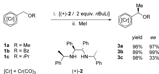
Scheme 1. Asymmetric functionalisation of tricarbonylchromium(0) ether complexes.
