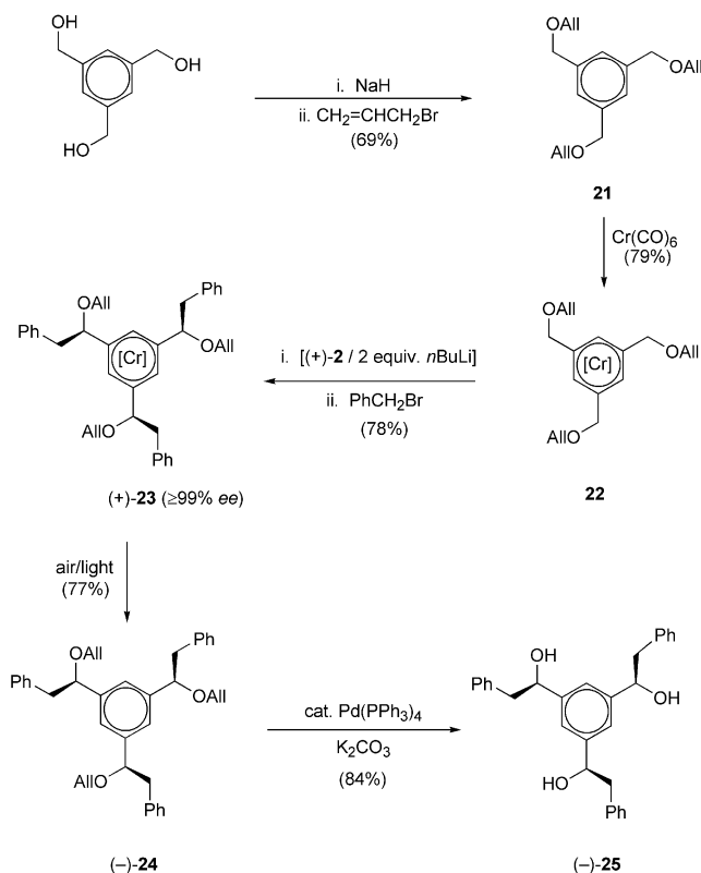
Scheme 6. Synthesis of an enantiopure triol.
